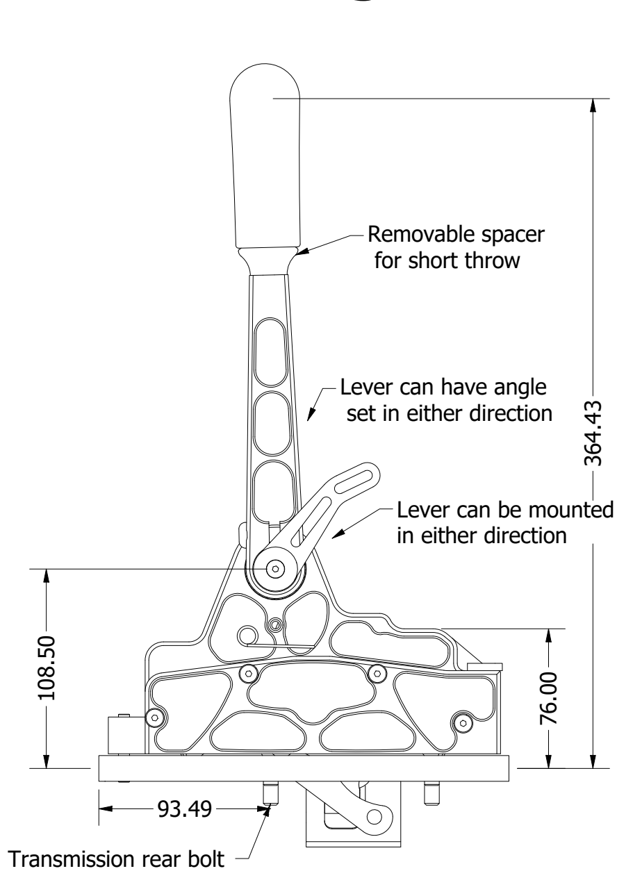
Side view
