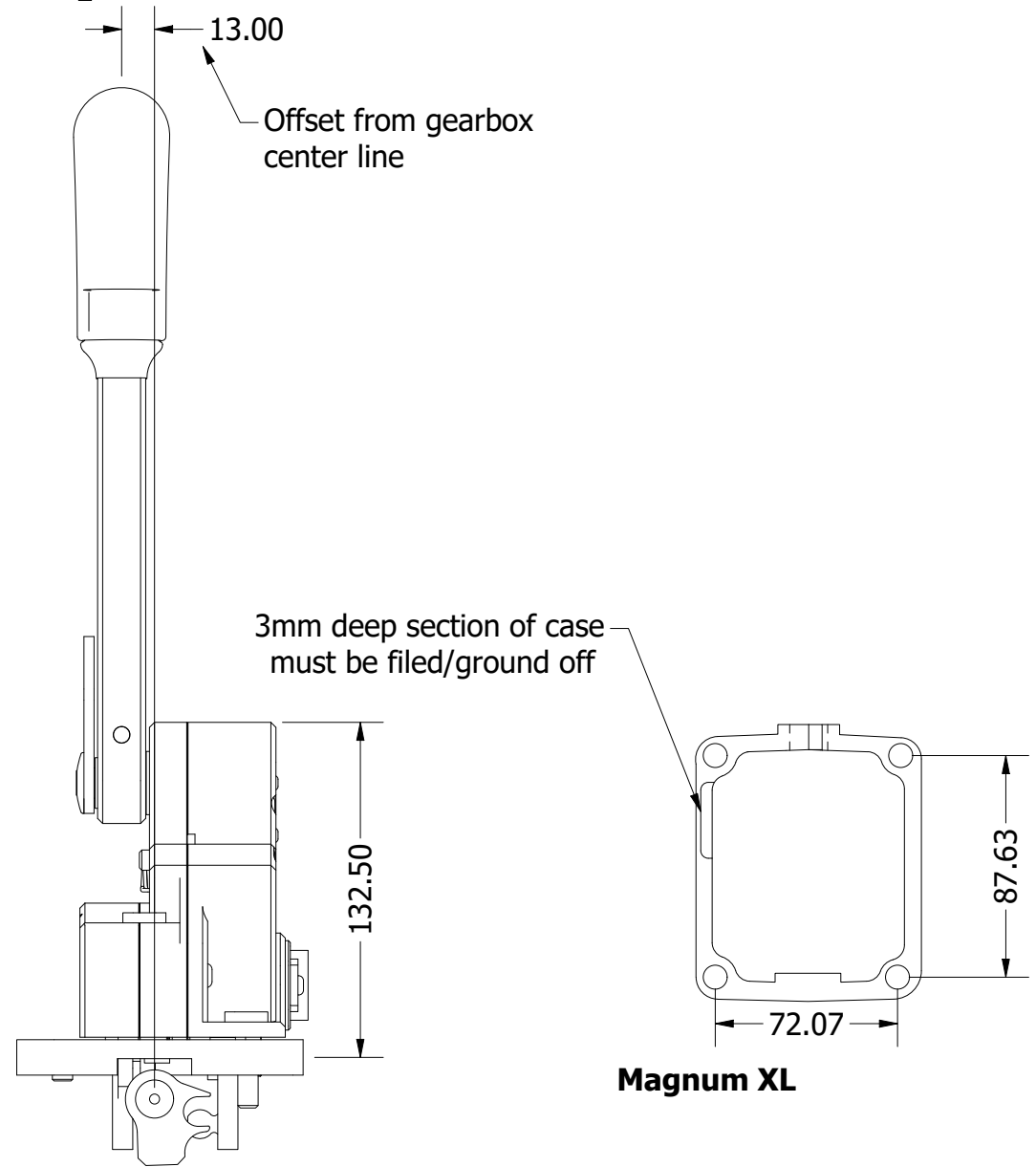
Front view
